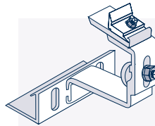
08 4 × Dachhaken
